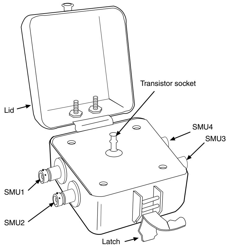
Figure 1 Test fixture
